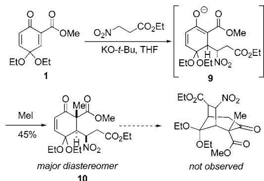
Scheme 1. Conjugate Addition and Methylation of 9 and Attempted Intramolecular Conjugate Addition of 10
